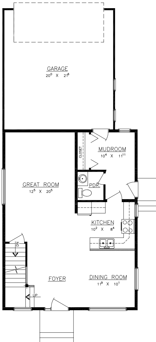
MAIN FLOOR AREA = 768 S.F.
